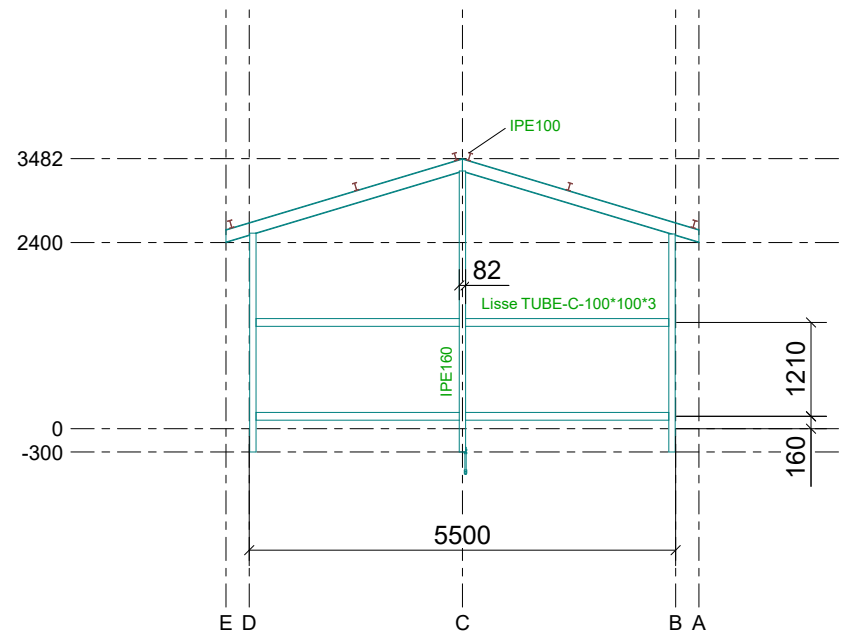
File 2 1:100
