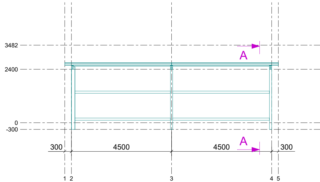
File B 1:100
